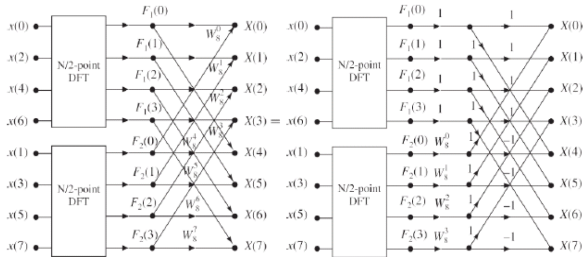
Figure 2.1 Illustration of flow graph of the first stage DIT FFT algorithm for N = 8 .
