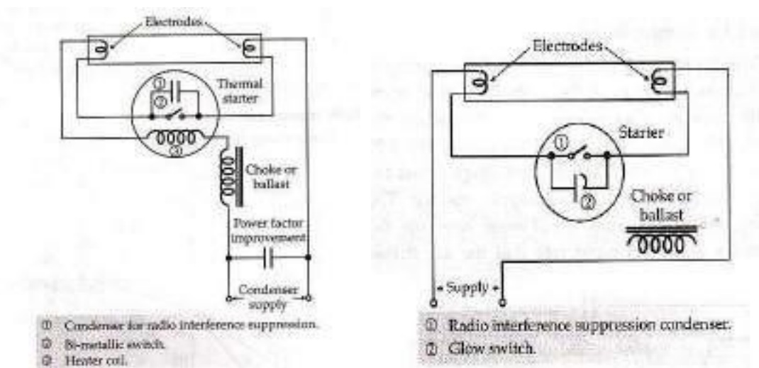
Fig.9 Fluorescent lamp
