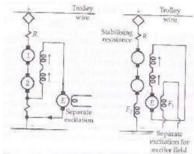
Fig. 23 Regenerative braking
