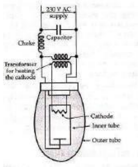
Fig.7 High pressure Mercury vapour Lamp
