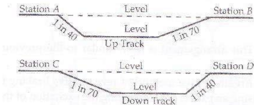
Fig.18 Track Grading
