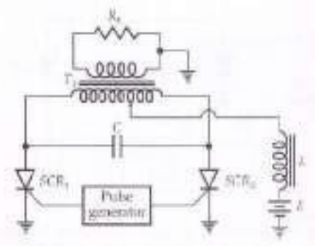
Fig. 19 Schematic of variable frequency inverter
