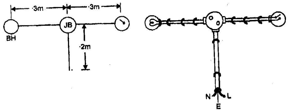
Fig. [II]:248. Showing conduit wiring
