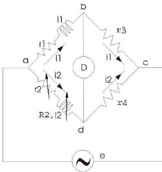
Maxwells Bridge
