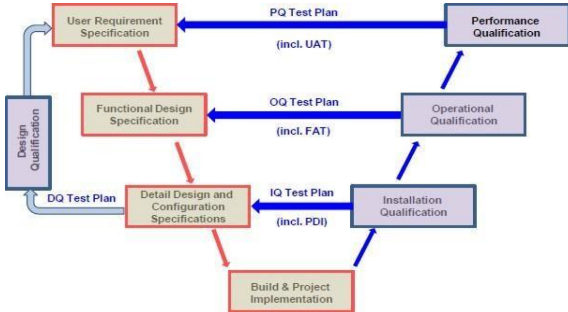
Figure 8 V-model
