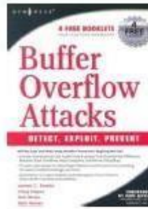
Memory corruption
