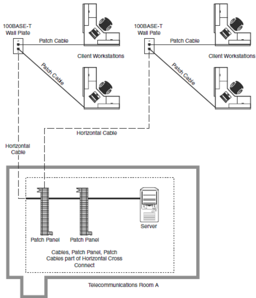
FIGURE 2.15 Horizontal cabling.
