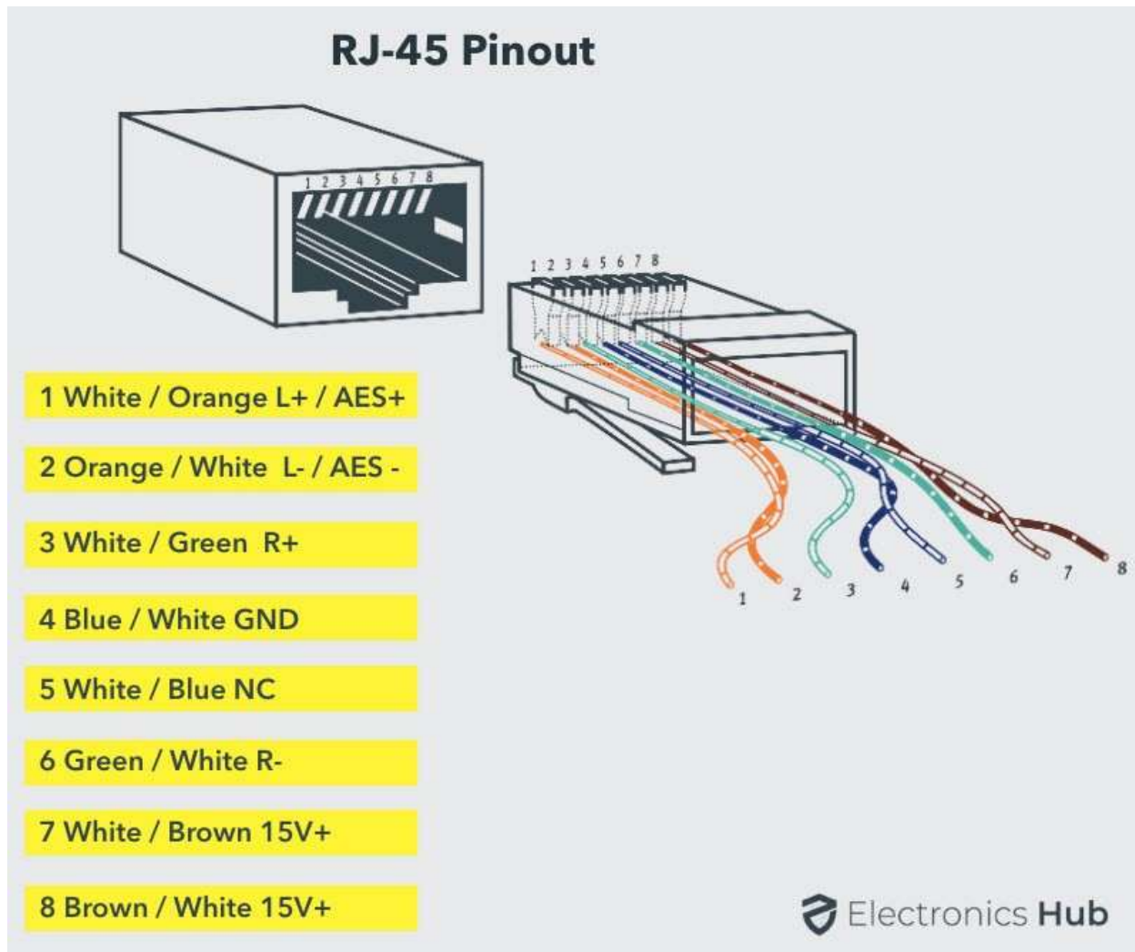
RJ-45-Connector-Pinout
